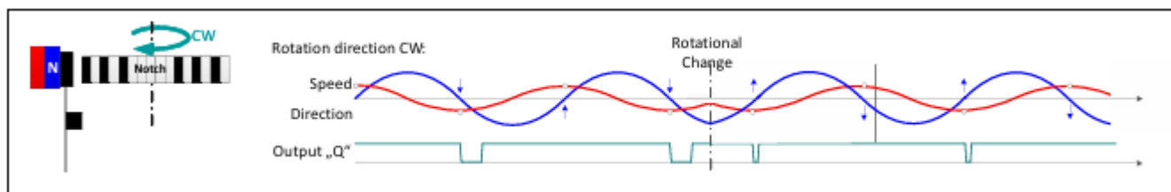
设置 “EDGE_POLAR = 1” 和 “FORWARD_DEF” = 1 时的信号输出
