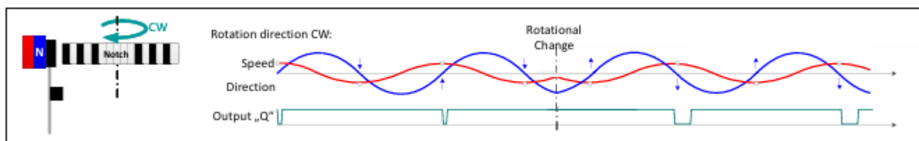
设置 “EDGE_POLAR = 1” 和 “FORWARD_DEF” = 0 时的信号输出
