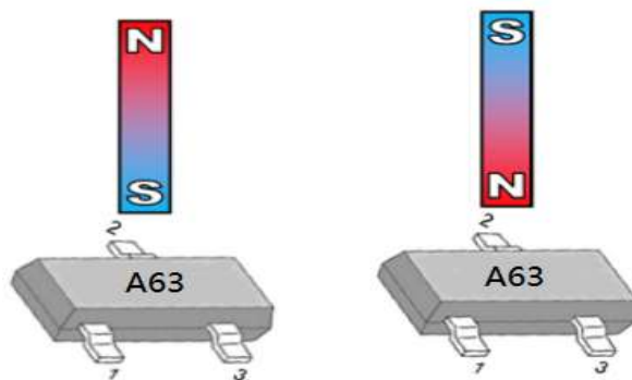
V_{OUT} =低电压 V_{OUT} =高电压 SOT23 (AH602)
